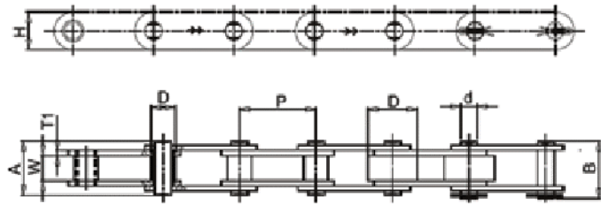
DOUBLE PITCH CONVEYOR CHAINS - AMERICAN SERIES
